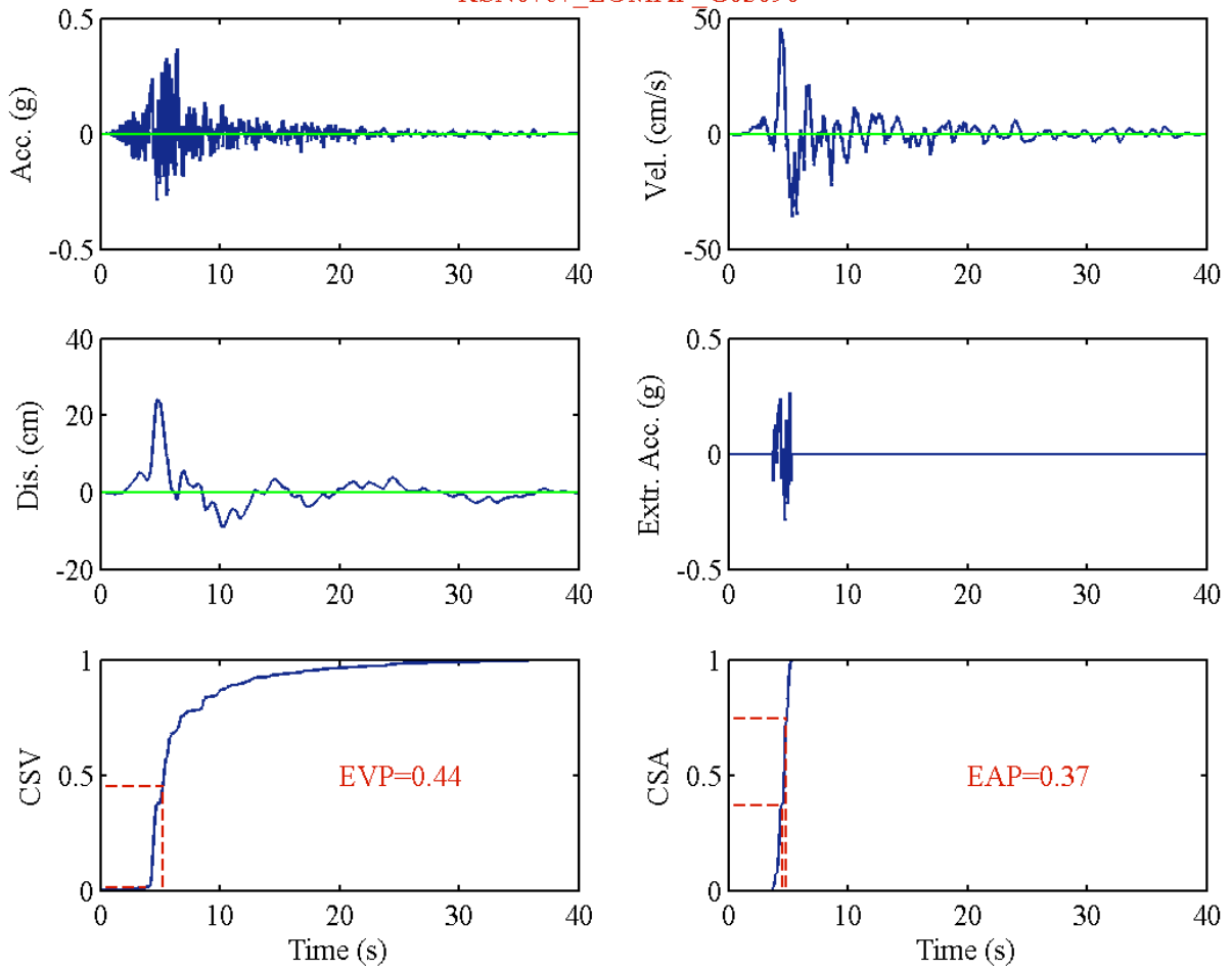
RSN0771_LOMAP_GGB270
