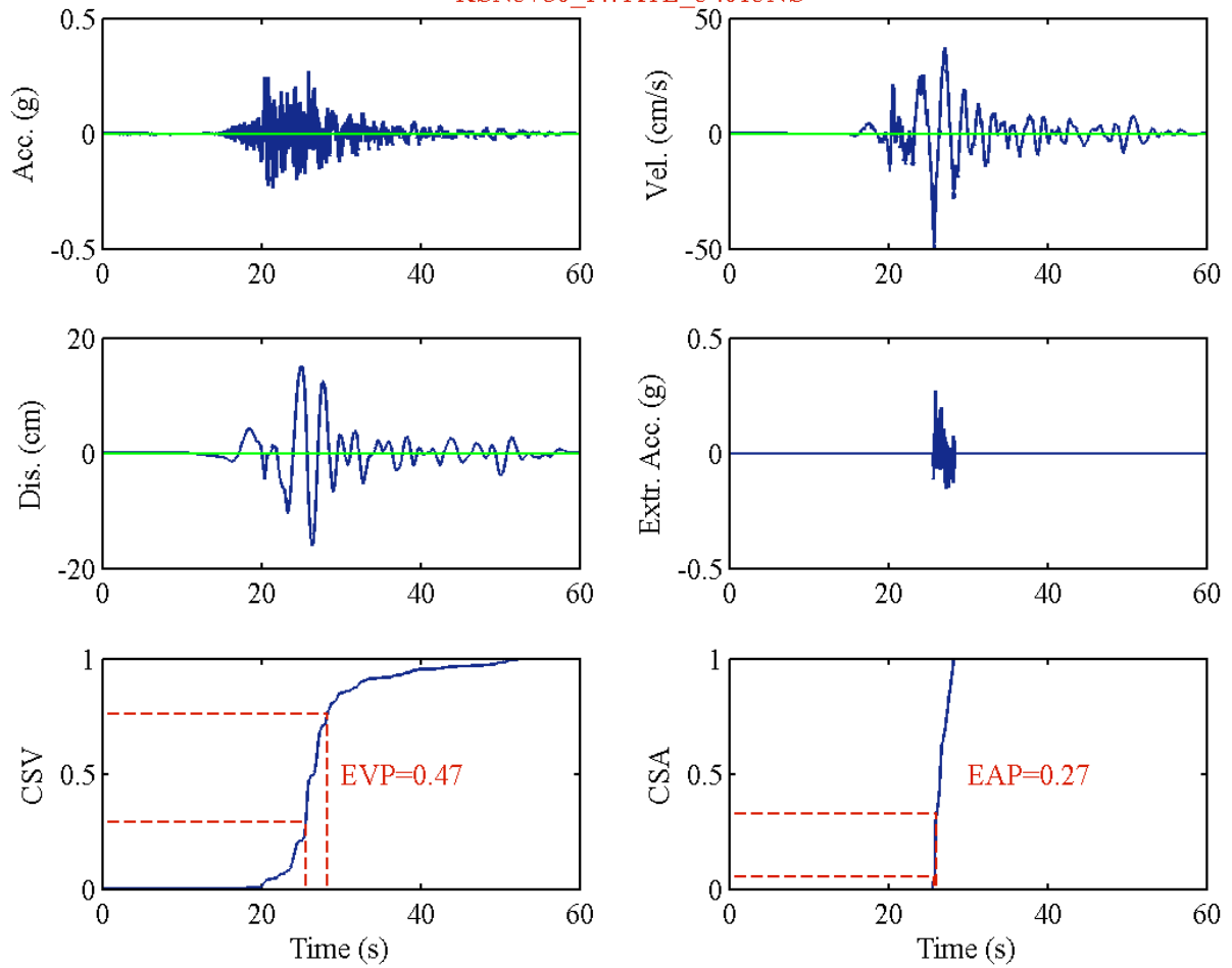
RSN5810_IWATE_56362EW
