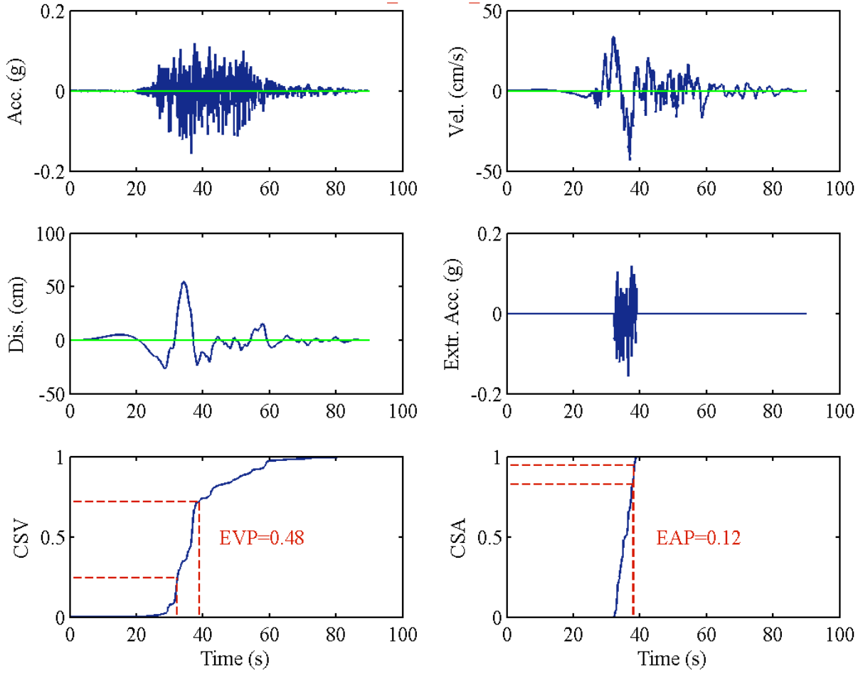
RSN1496_CHICHI_TCU056-E
