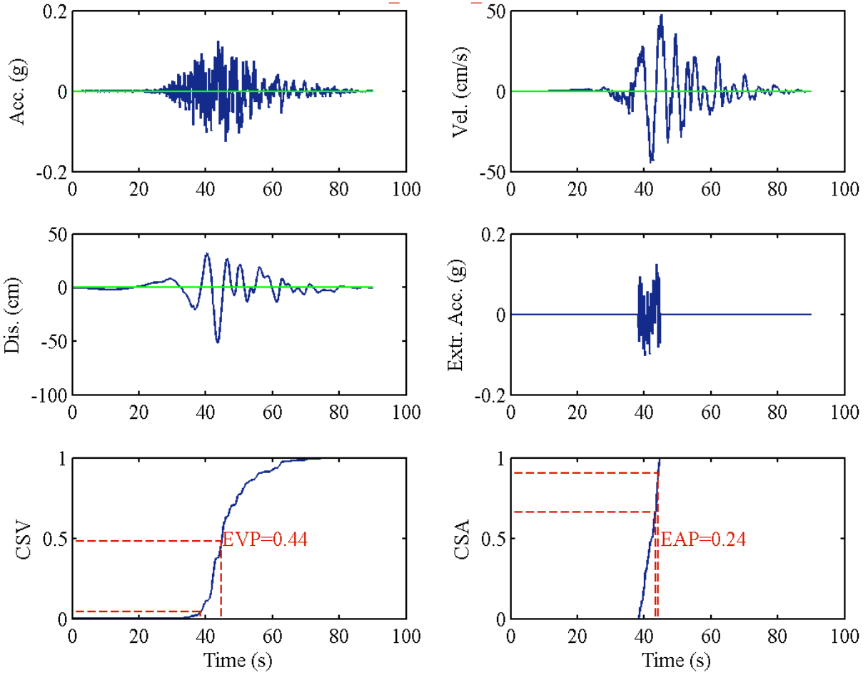
RSN1481_CHICHI_TCU038-E
