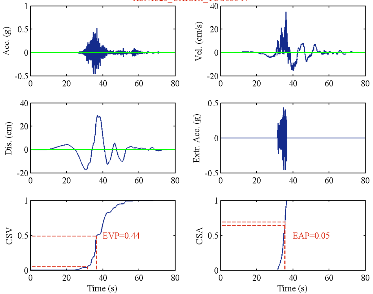
RSN1520_CHICHI_TCU088-N
