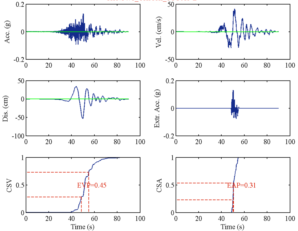
RSN1471_CHICHI_TCU015-E
