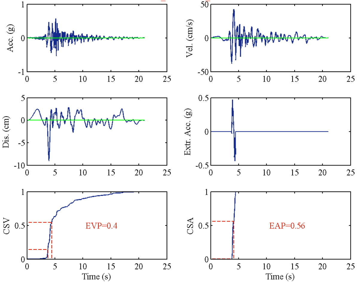
RSN4116_PARK2004_Z14360
