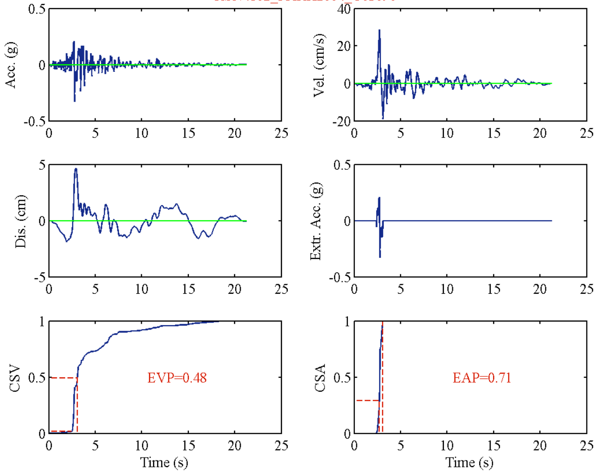
RSN4102_PARK2004_C03090
