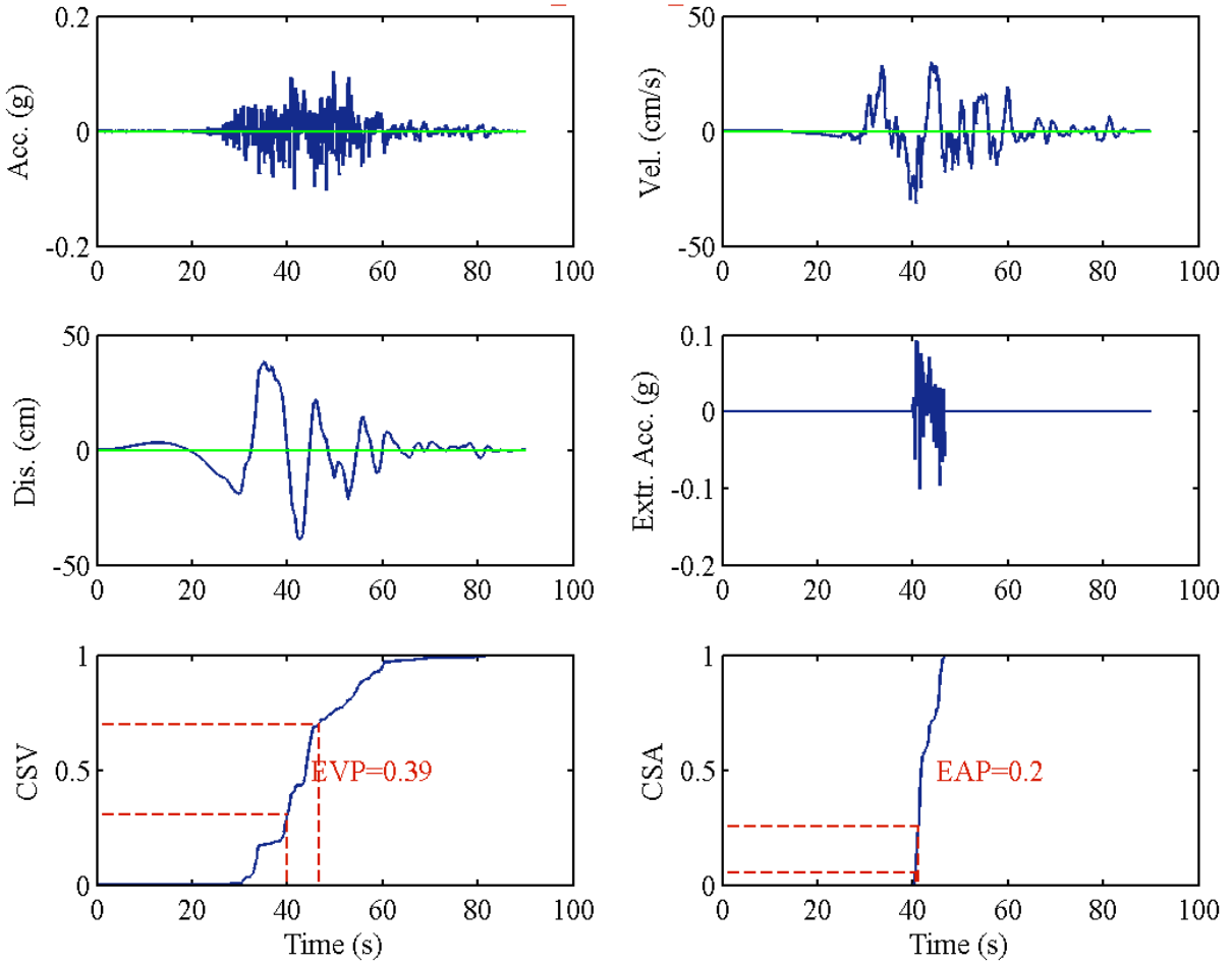
RSN1531_CHICHI_TCU104-E
