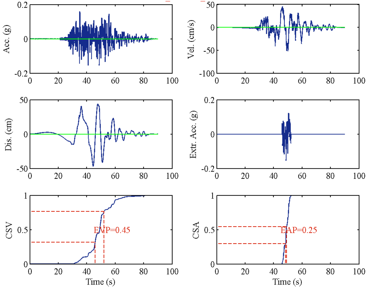
RSN1498_CHICHI_TCU059-E
