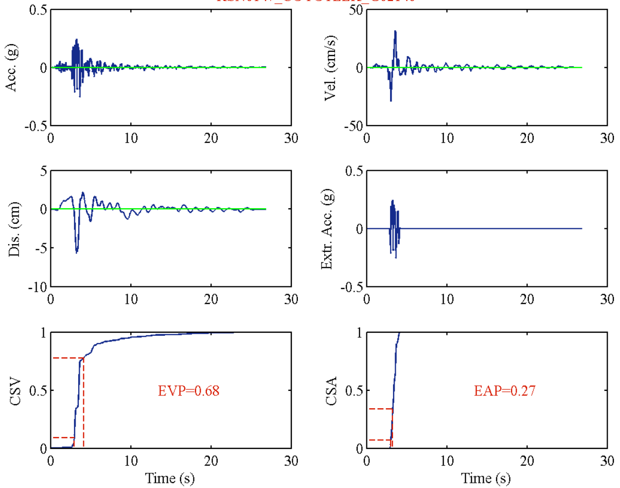
RSN0149_COYOTELK_G04360
