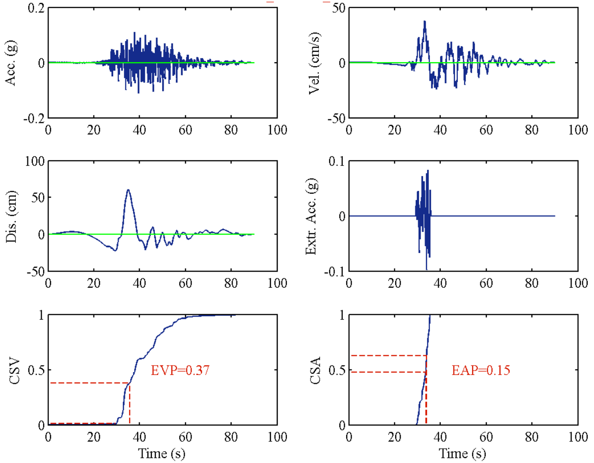
RSN1527_CHICHI_TCU100-E
