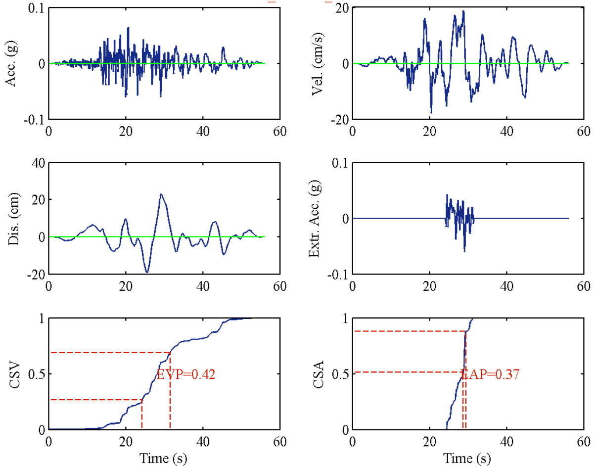
RSN1471_CHICHI_TCU015-E
