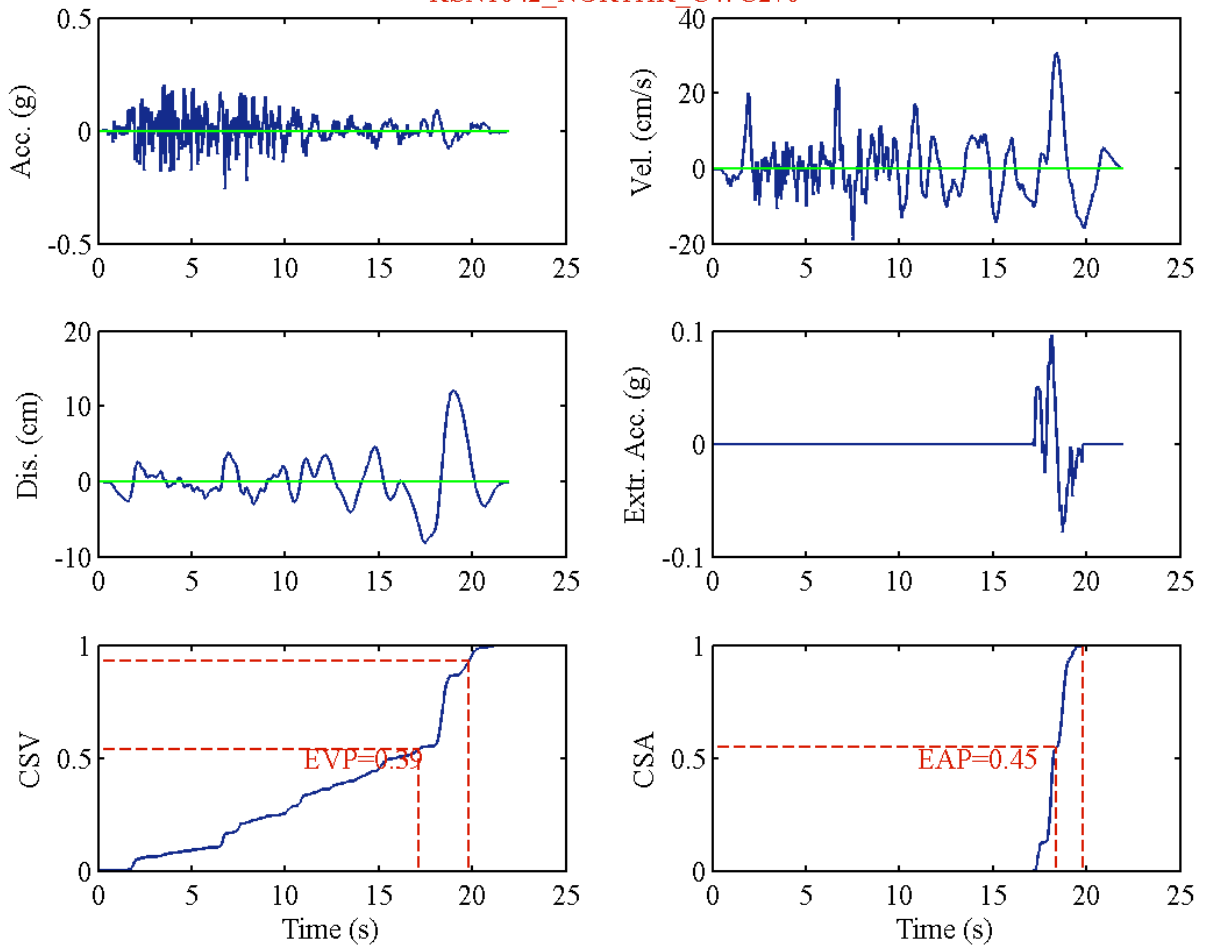
RSN1045_NORTHR_WPI046
