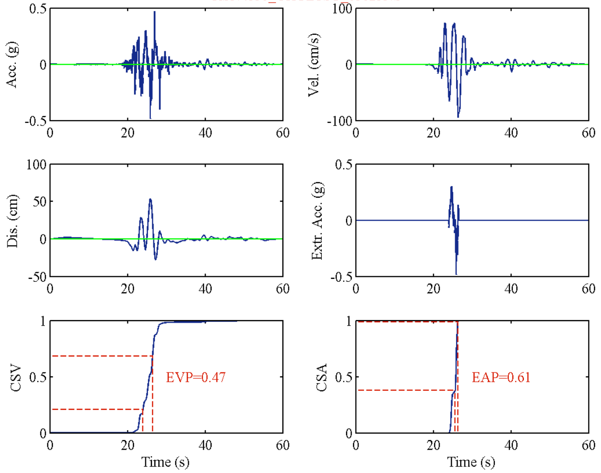
RSN4875_CHUETSU_65058EW
