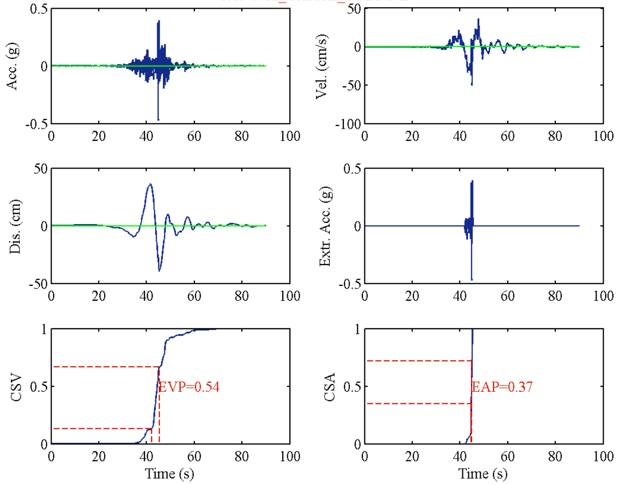
RSN1485_CHICHI_TCU045-E
