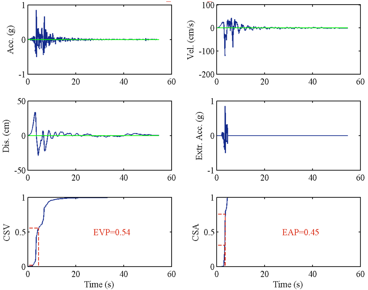
RSN1085_NORTHR_SCE011
