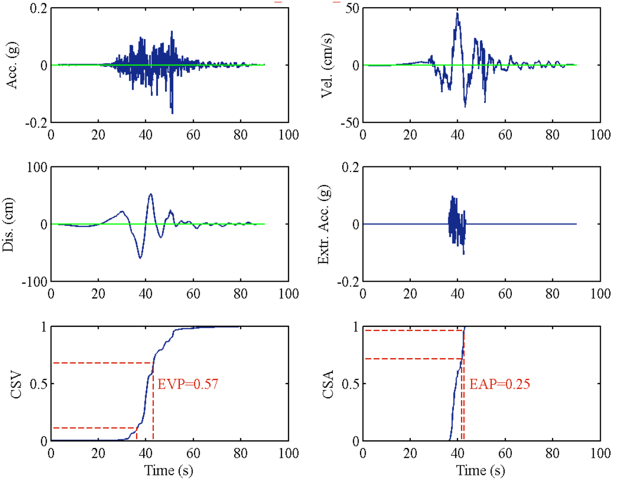
RSN1555_CHICHI_TCU147-E
