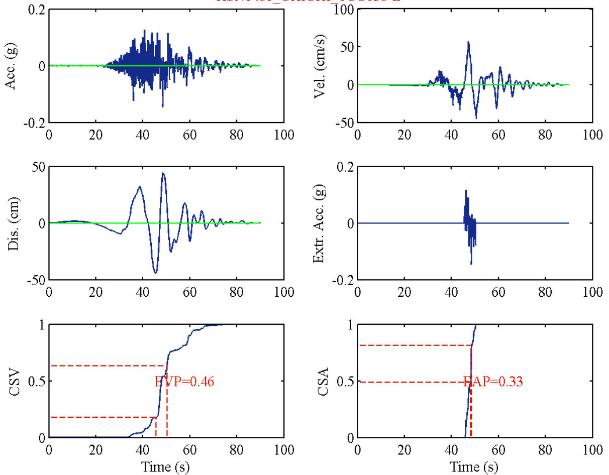
RSN1481_CHICHI_TCU038-E
