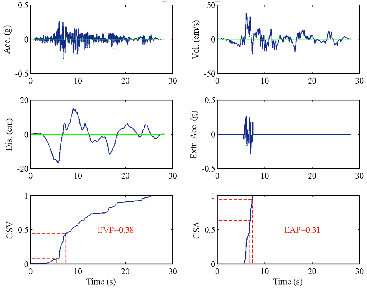
RSN3750_CAPEMEND_LFS360
