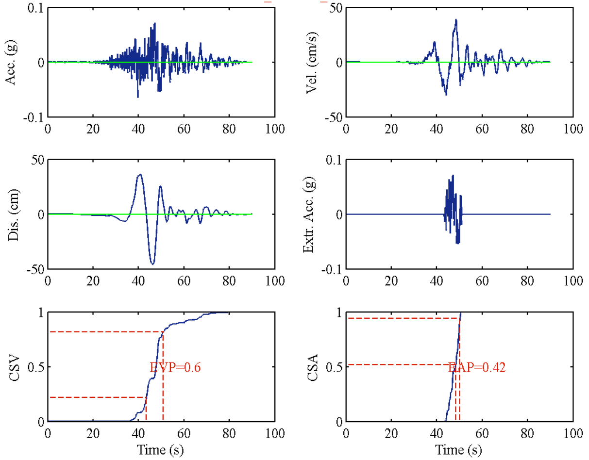
RSN1523_CHICHI_TCU094-N
