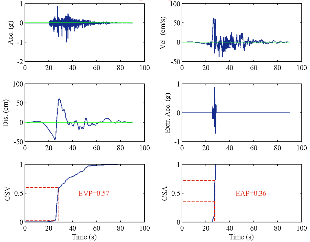
RSN1550_CHICHI_TCU136-N
