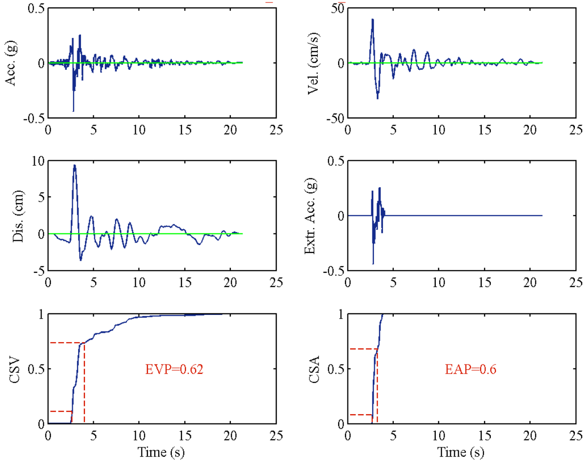
RSN4098_PARK2004 C01090
