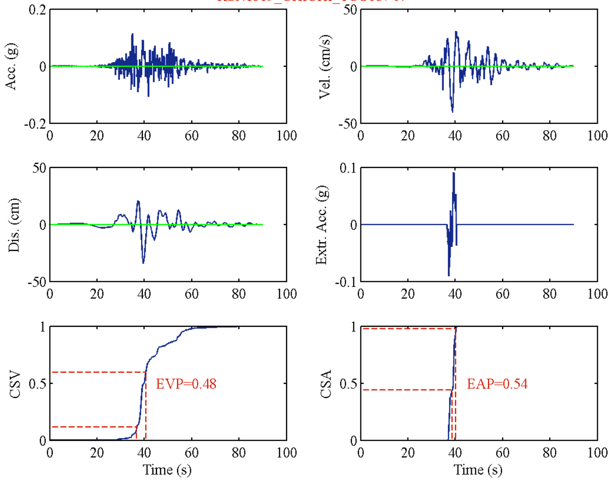
RSN1520_CHICHI_TCU088-N
