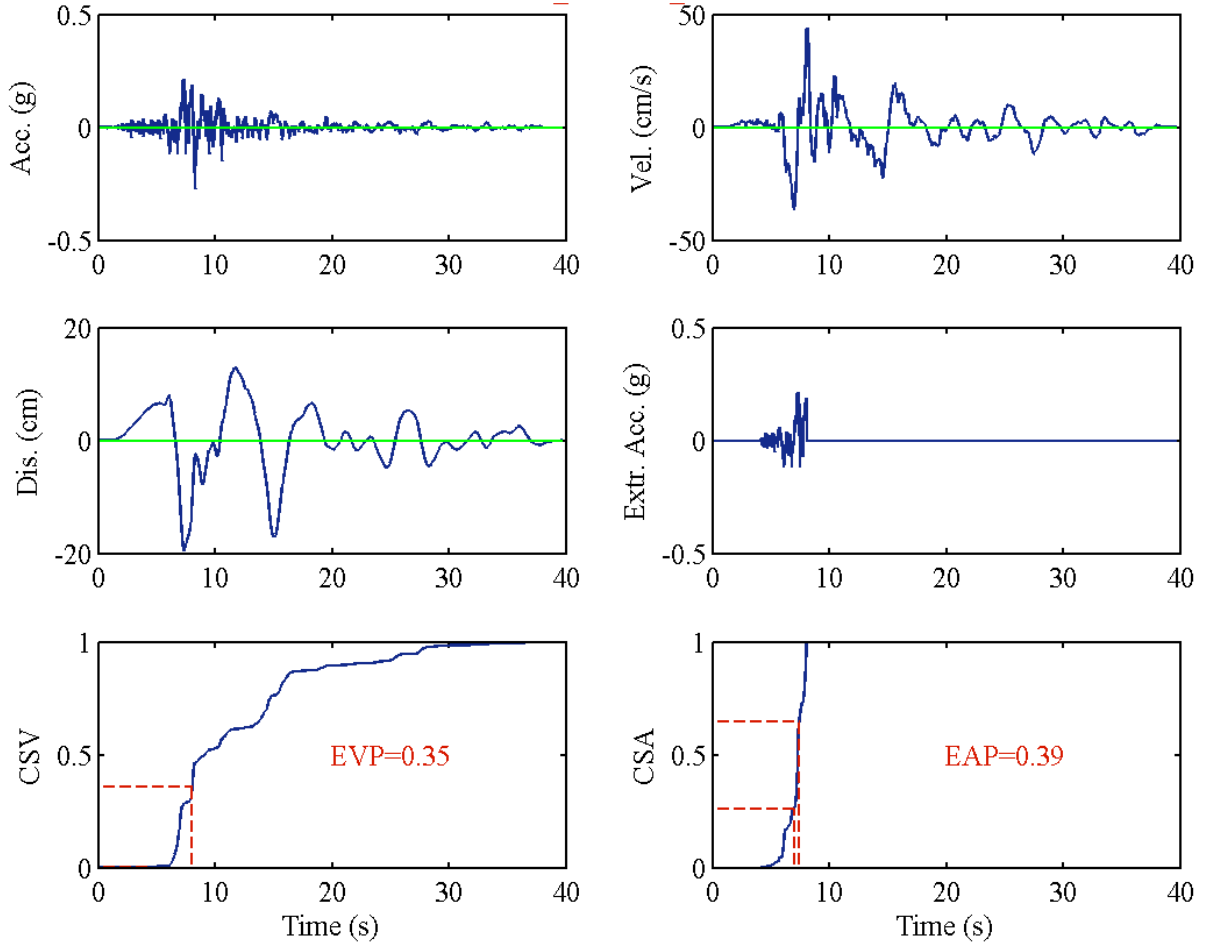
RSN0778_LOMAP_HDA165
