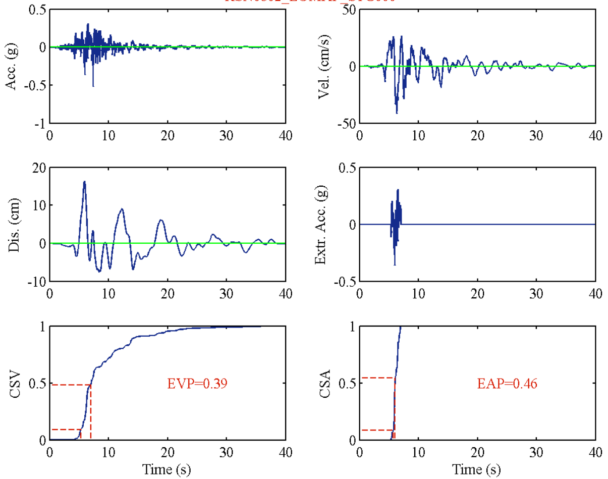
RSN0802_LOMAP_STG090
