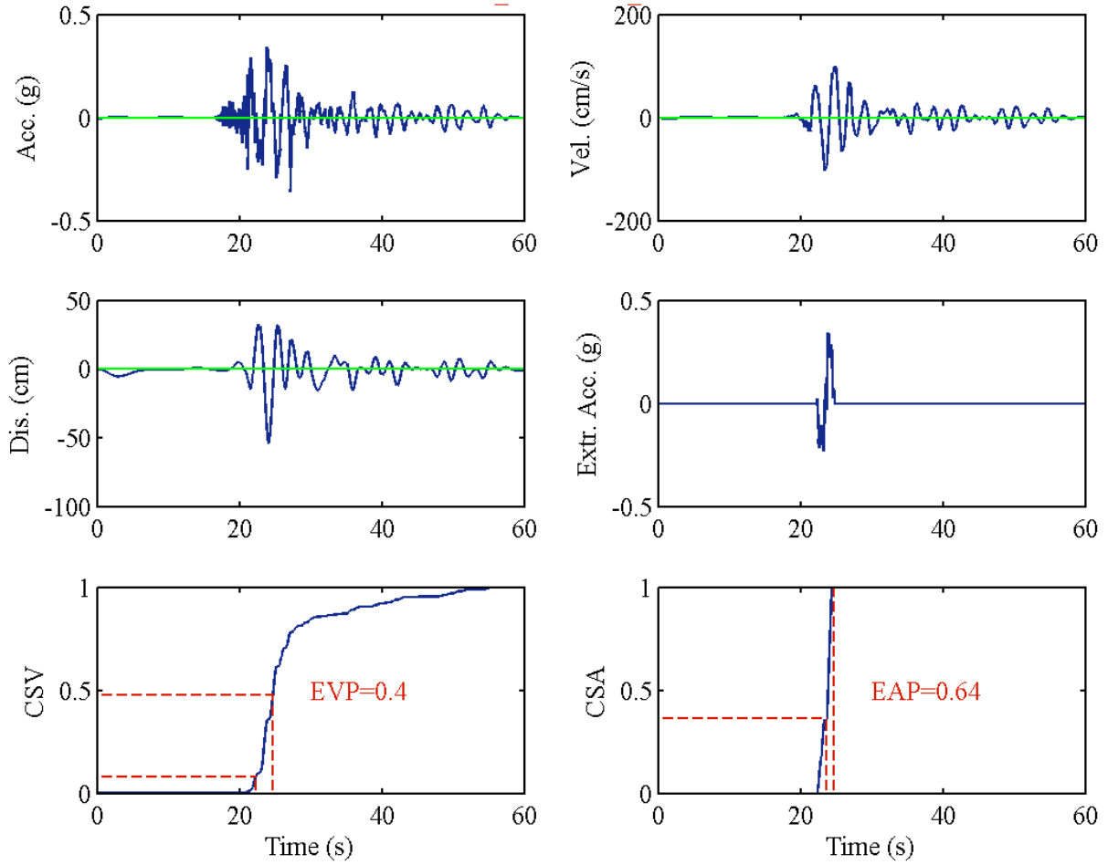
RSN4875_CHUETSU_65058EW
