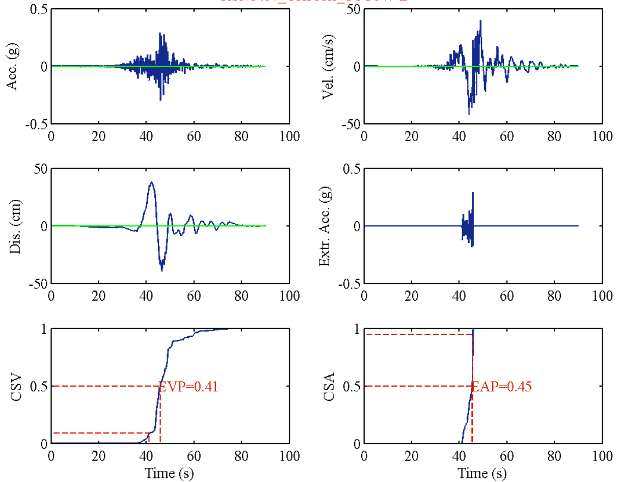
RSN1487_CHICHI_TCU047-E
