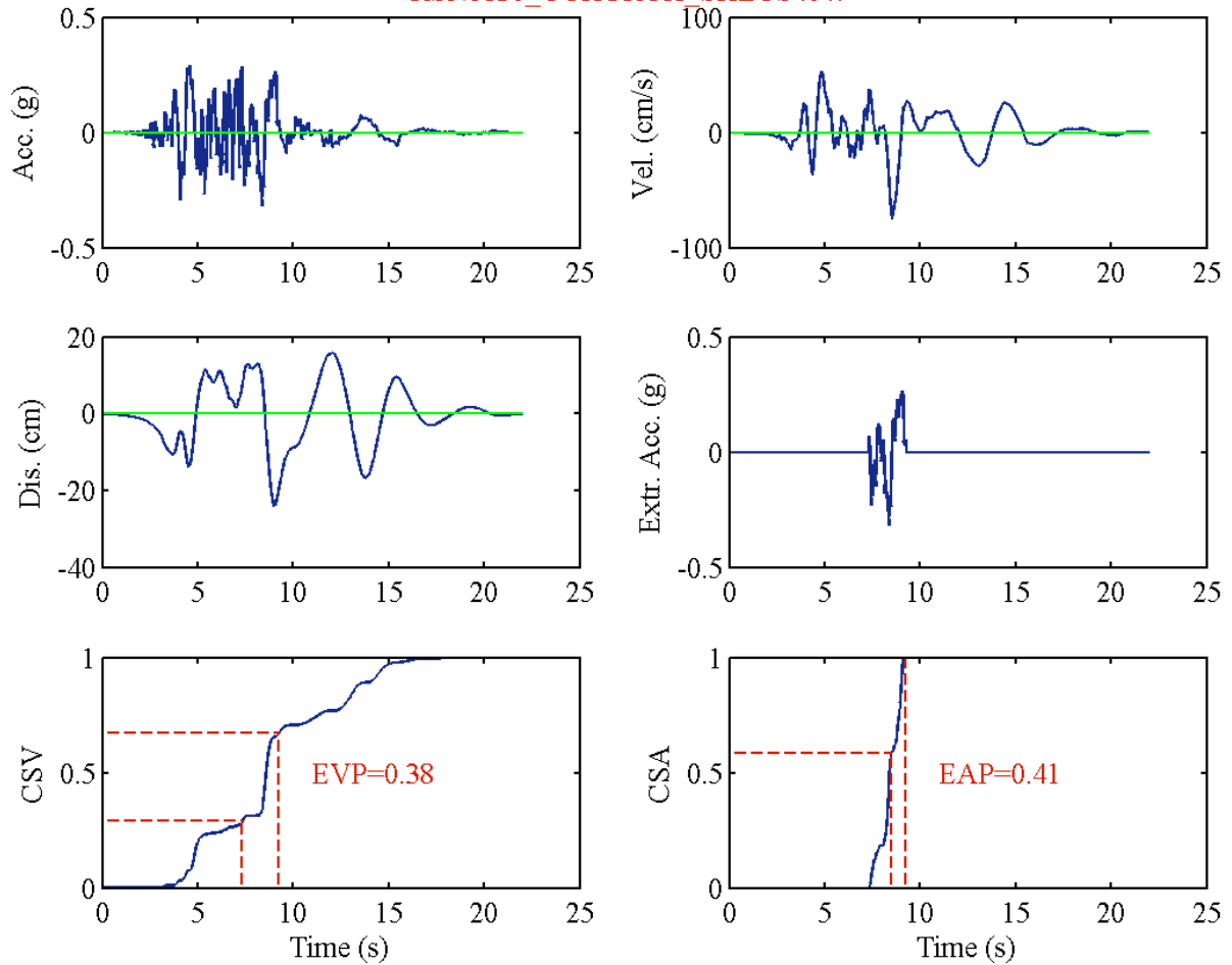
RSN8130_CCHURCH_SHLCS40W
