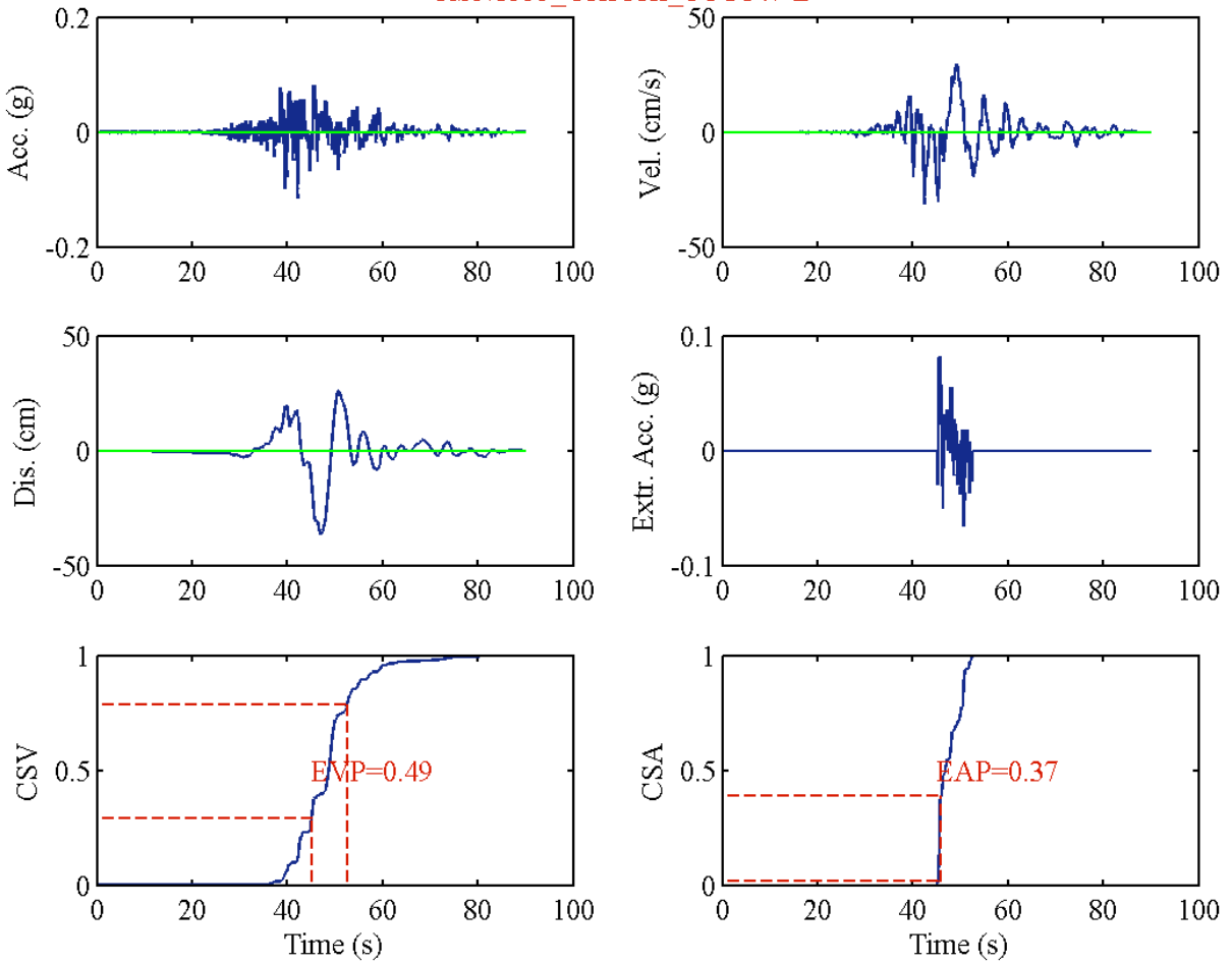
RSN1555_CHICHI_TCU147-E
