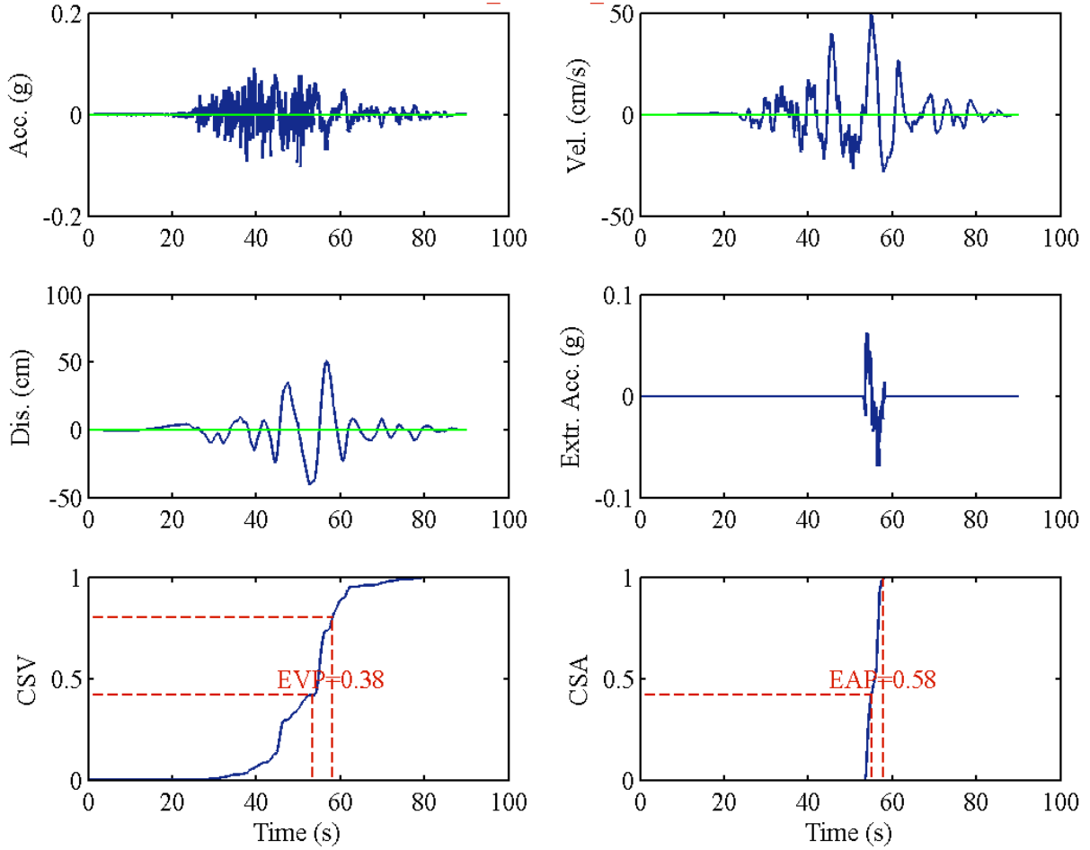
RSN1498_CHICHI_TCU059-E
