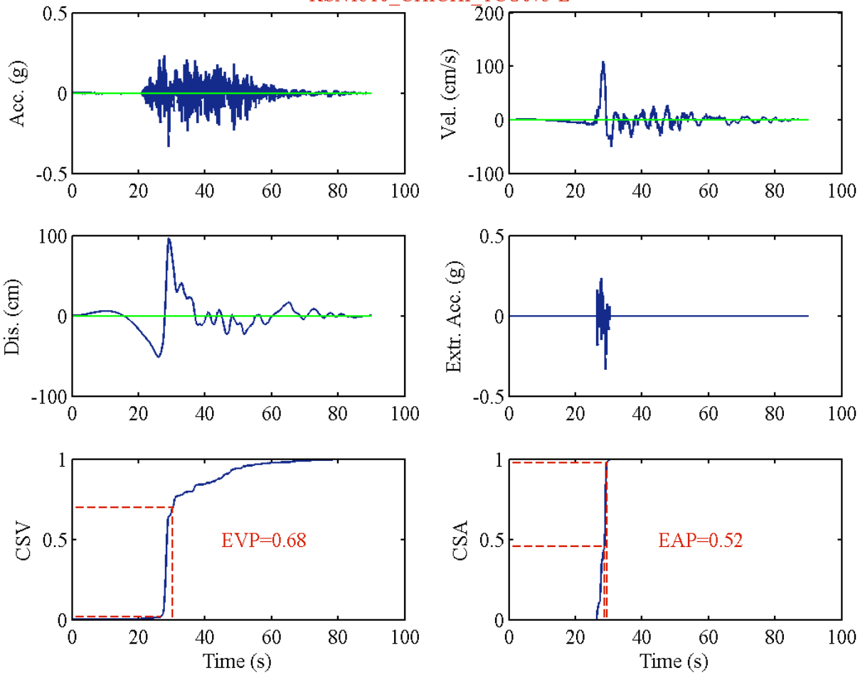
RSN1511_CHICHI_TCU076-E
