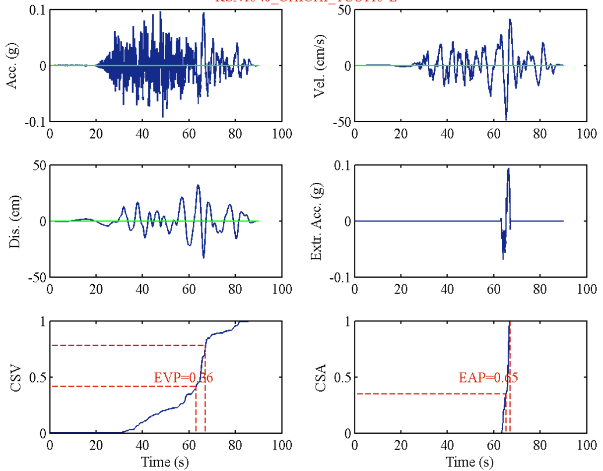
RSN1540_CHICHI_TCU115-E
