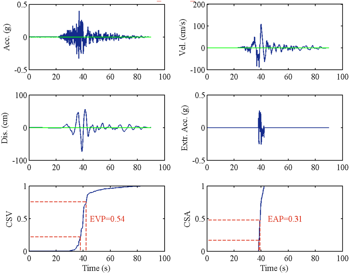
RSN1244_CHICHI_CHY101-N
