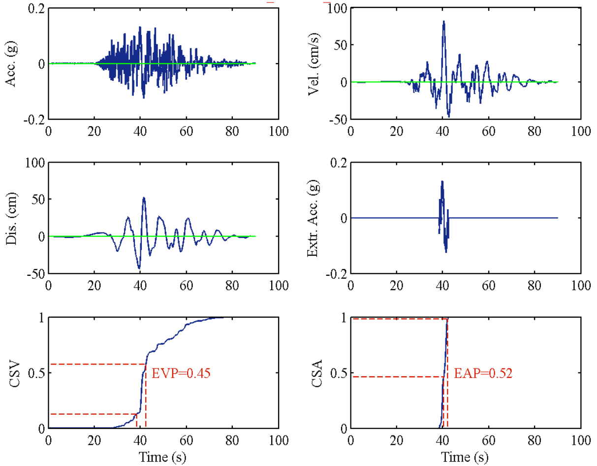
RSN1501_CHICHI_TCU063-N
