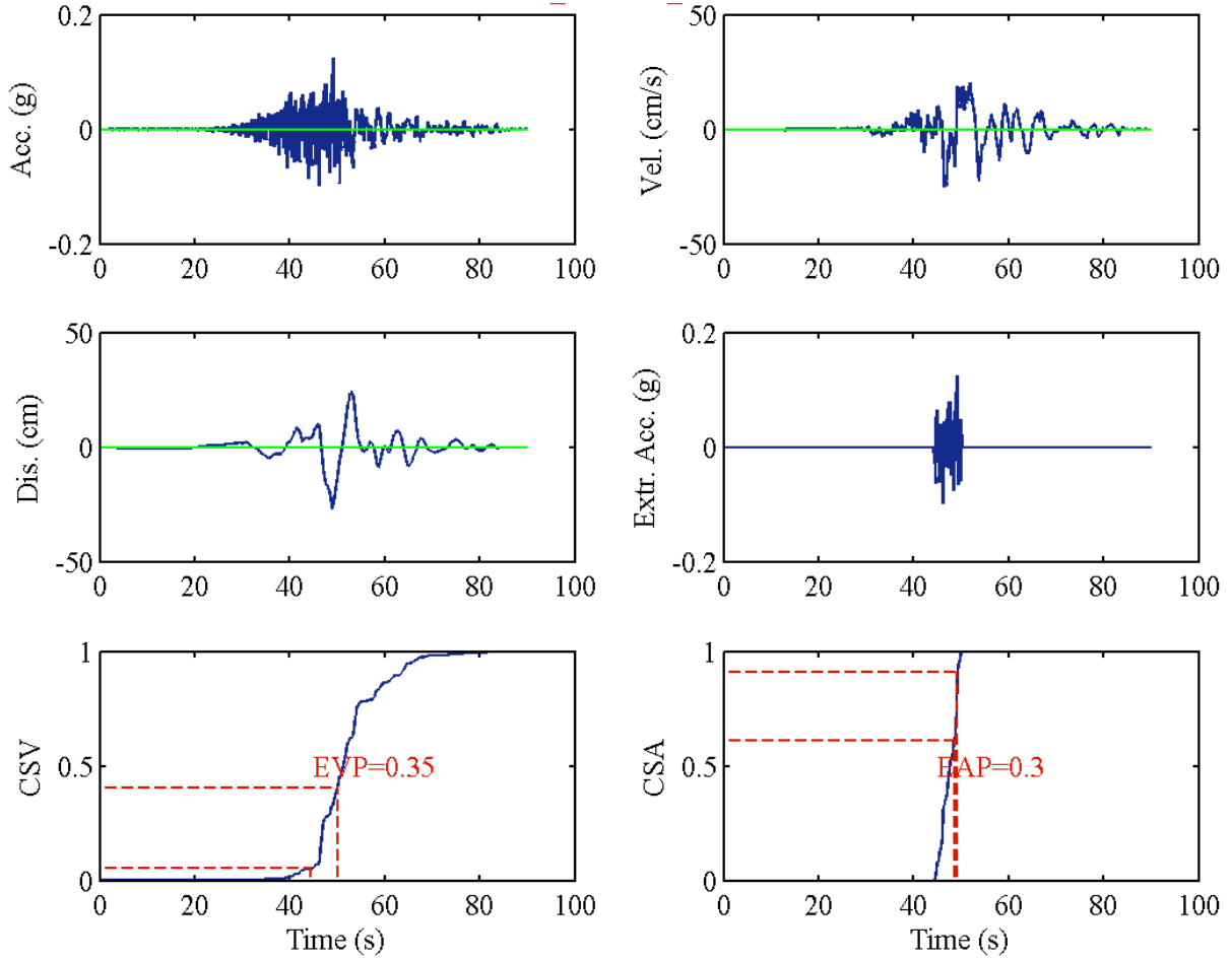
RSN1471_CHICHI_TCU015-N
