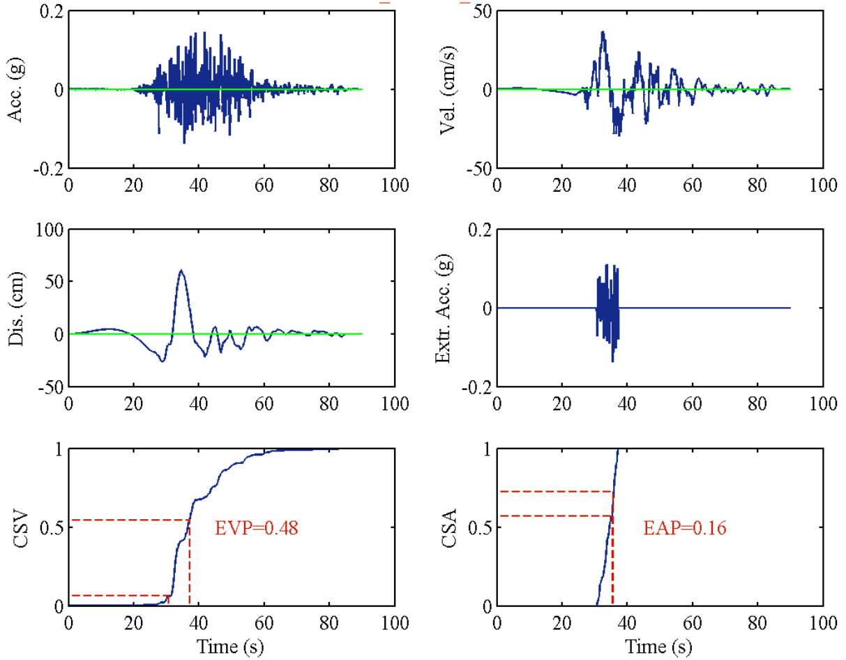
RSN1490_CHICHI_TCU050-E
