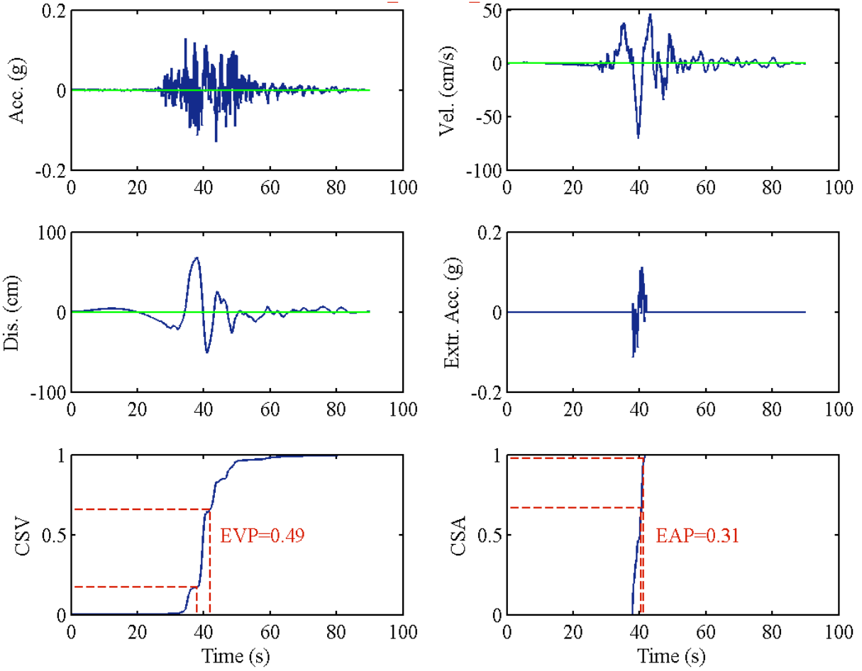
RSN1530_CHICHI_TCU103-E
