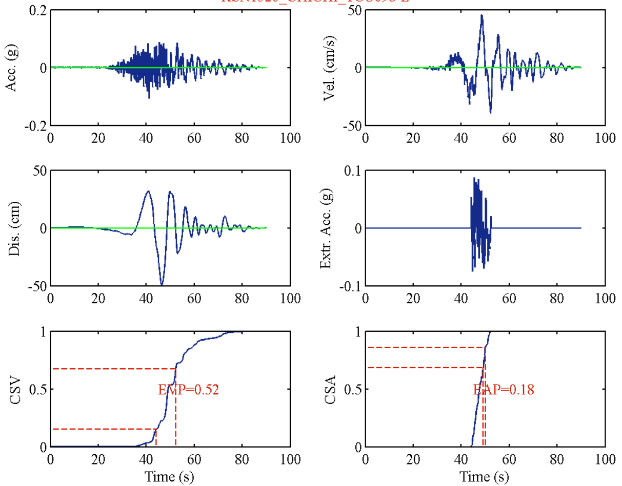
RSN1526_CHICHI_TCU098-E
