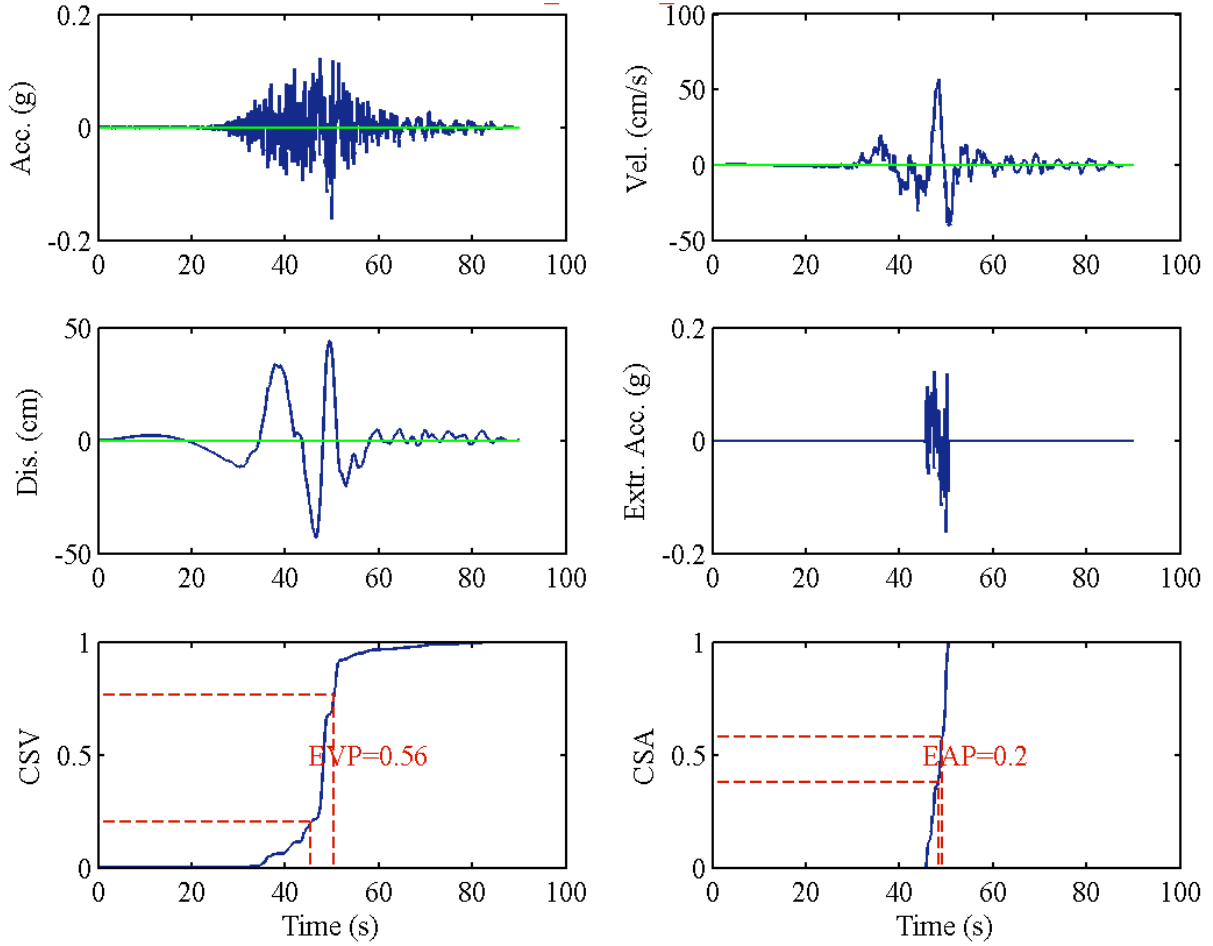
RSN1483_CHICHI_TCU040-E
