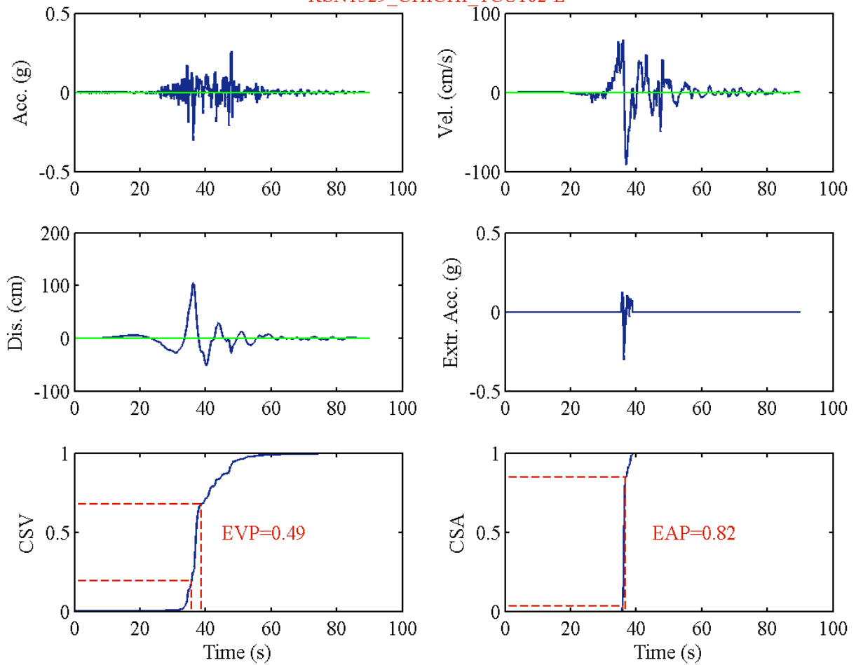
RSN1529_CHICHI_TCU102-E
