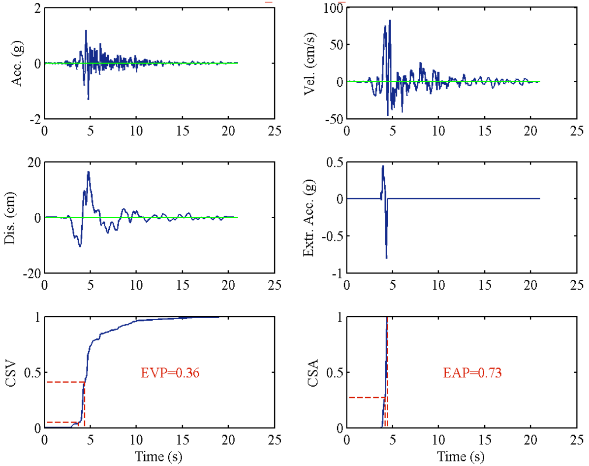
RSN4116_PARK2004_Z14090
