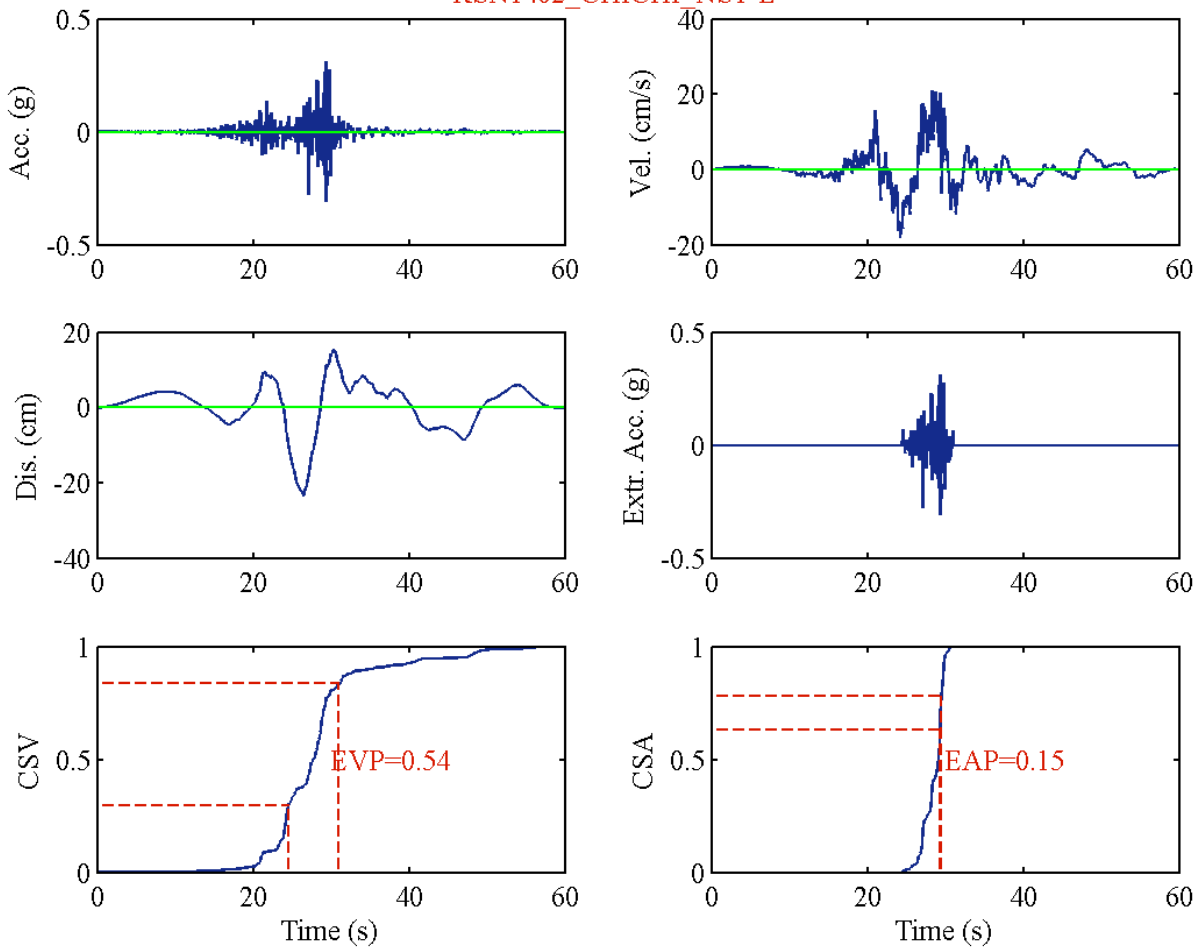
RSN1402_CHICHI_NST-E
