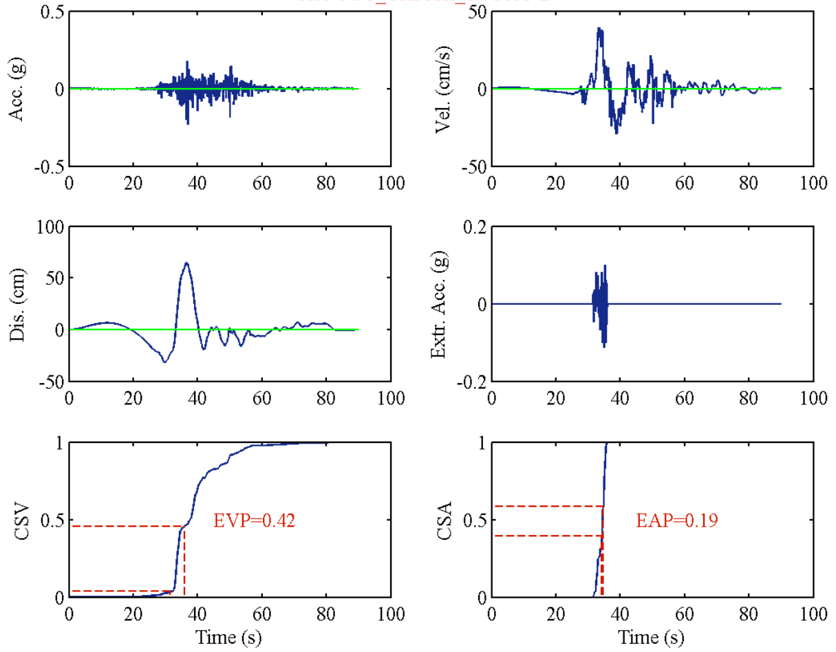
RSN1494_CHICHI_TCU054-E
