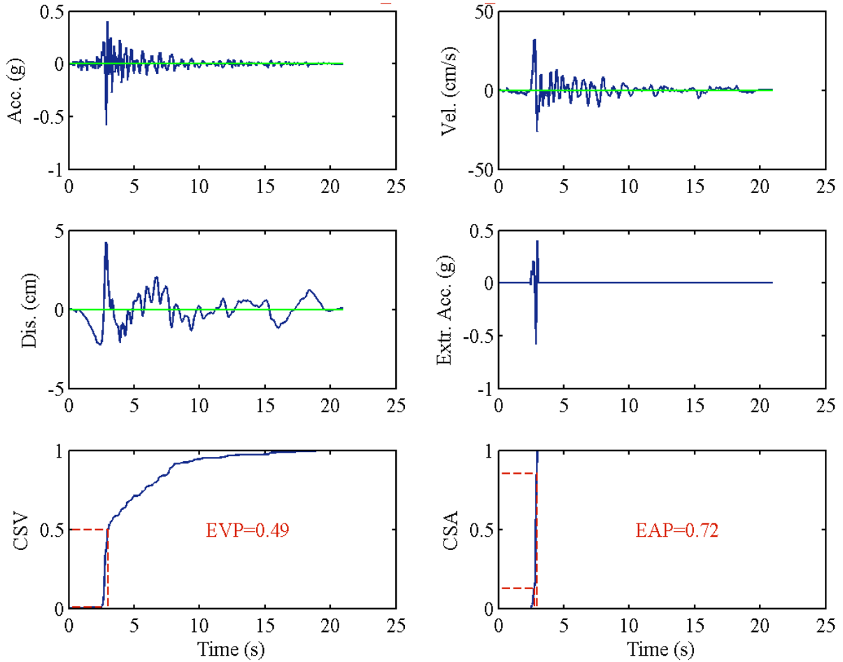
RSN4103_PARK2004_C04090
