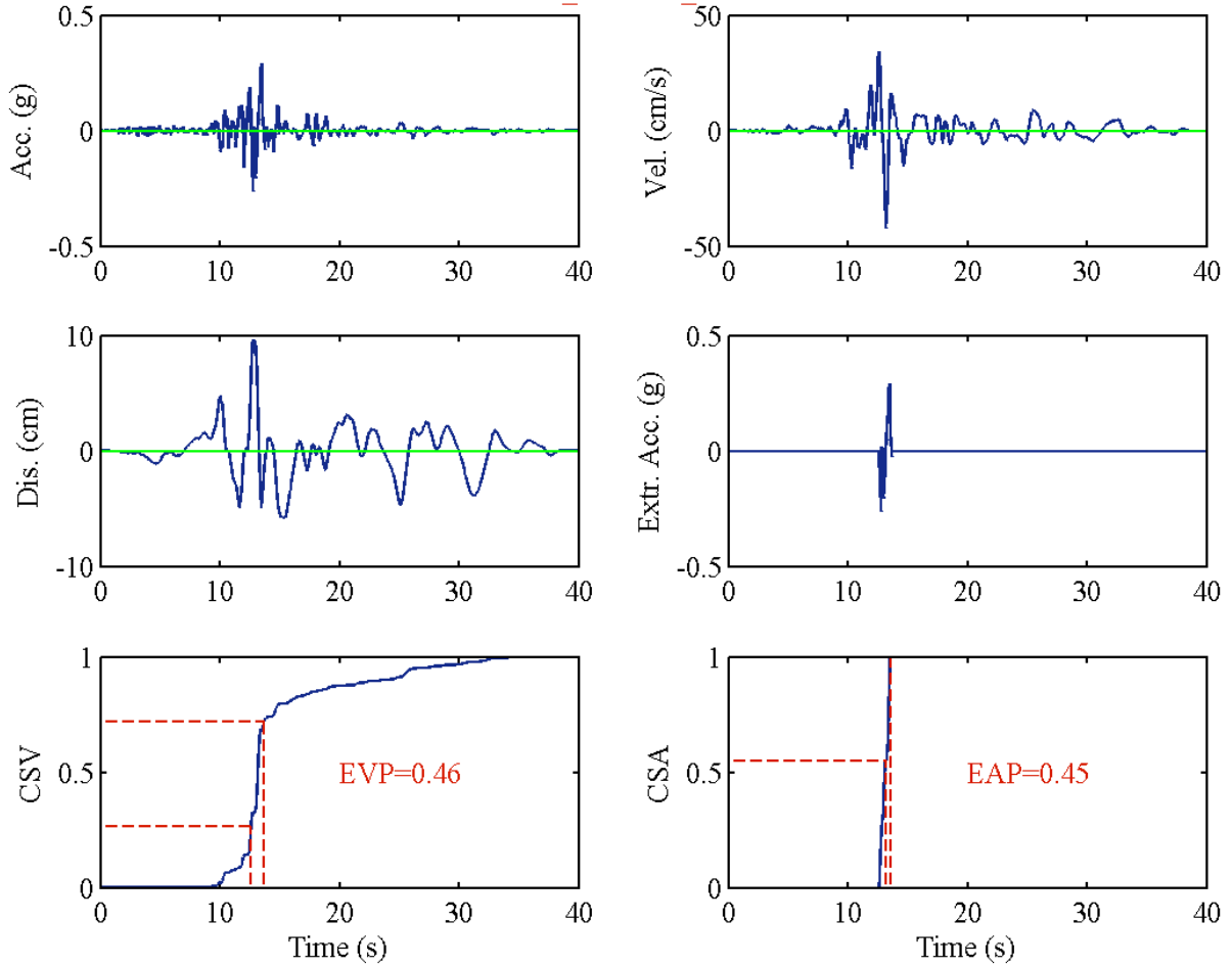
RSN0783_LOMAP_OHW000
