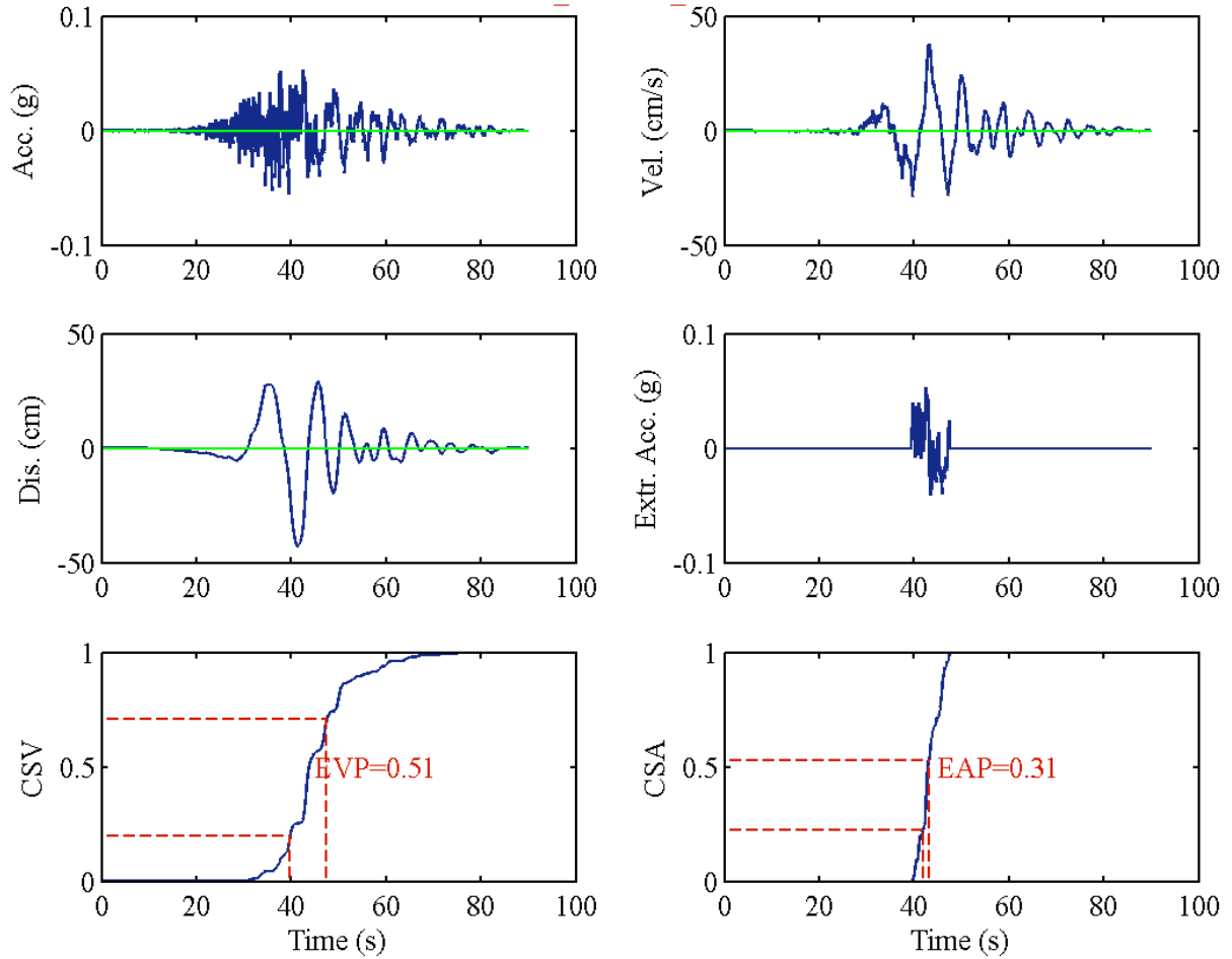
RSN1525_CHICHI_TCU096-E
