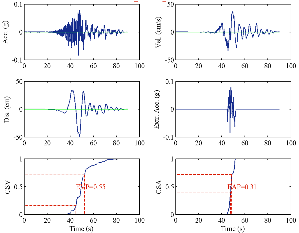
RSN1472_CHICHI_TCU017-E
