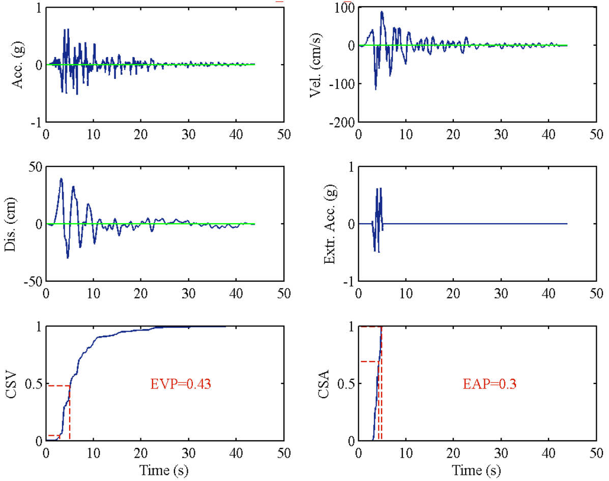
RSN1084_NORTHR_SCS052
